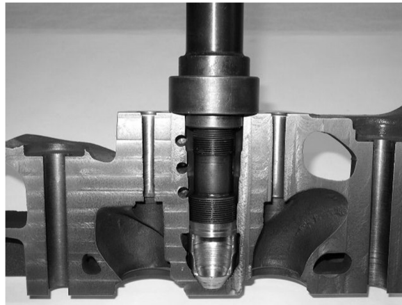
Sleeve Remover
